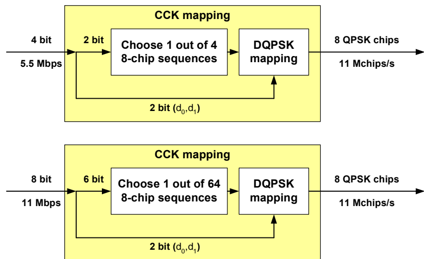
Figure 7 – 802.11b 5.5/11 Mbit/s operation
