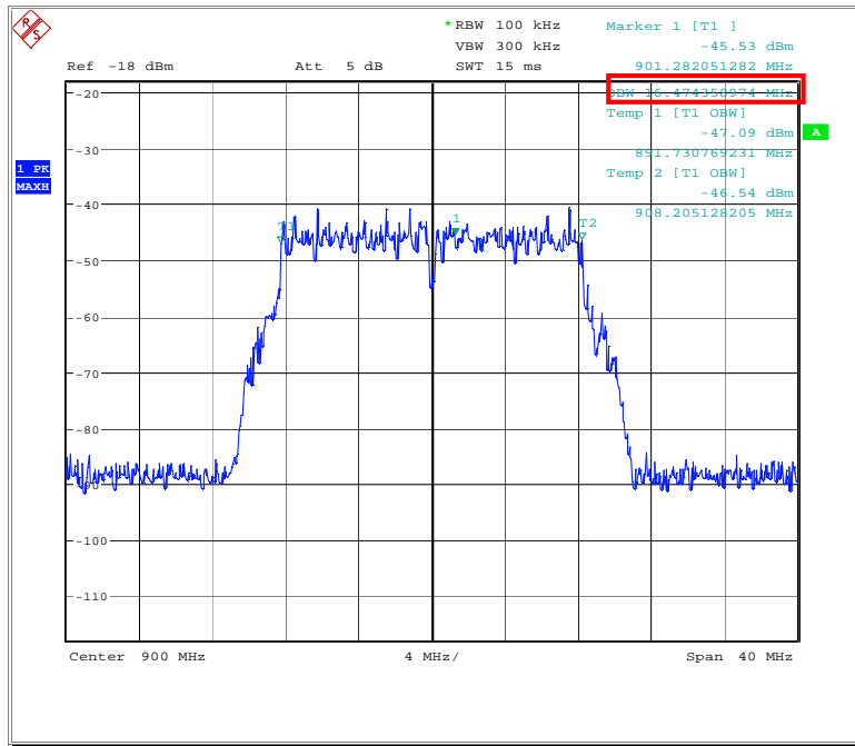
Figure 11 – Occupied bandwidth typical measurement result
