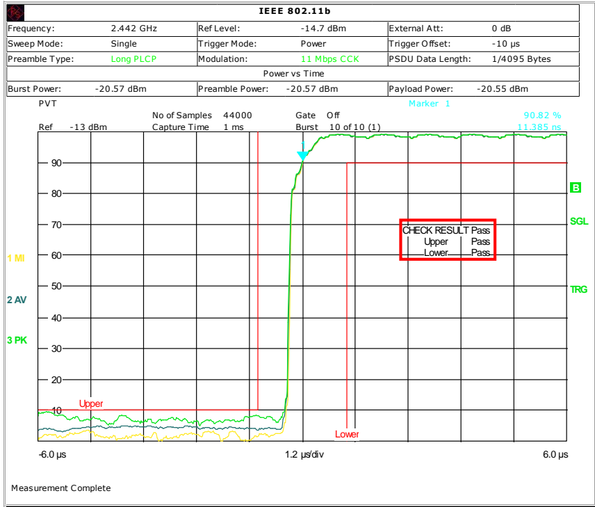
Figure 31 – Transmit power ramp typical measurement result (power-up ramp)
