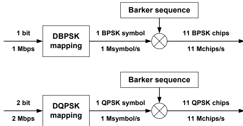
Figure 6 – 802.11b 1/2 Mbit/s operation
