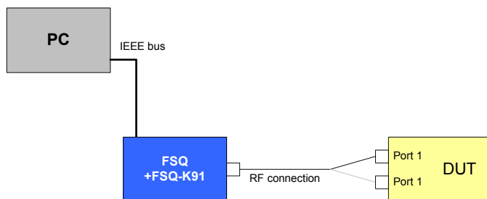
Drawing 20 – Transmit center frequency tolerance test setup
