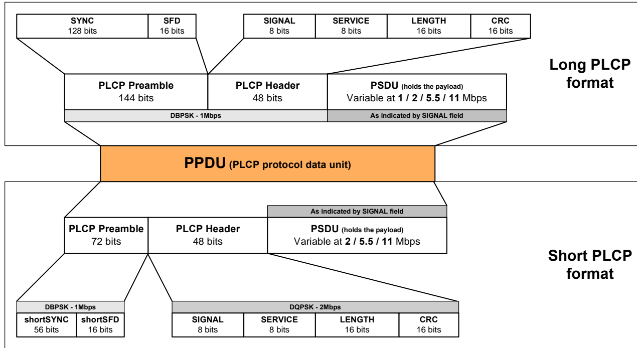
Figure 9 – 802.11b packet format
