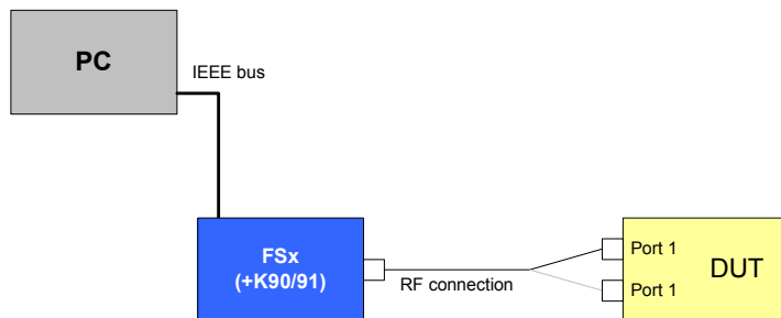
Drawing 4 – Transmit spectrum mask test setup
