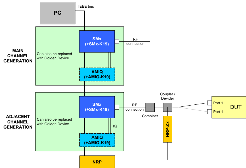
Drawing 14 – Non-adjacent channel rejection test setup
