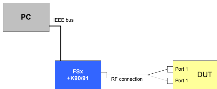
Drawing 8 – Center frequency leakage test setup
