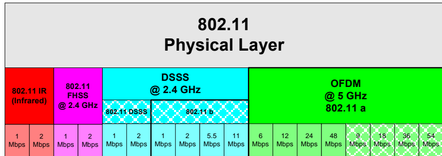
Figure 3 – Overview over standardized 802.11 physical layer systems
