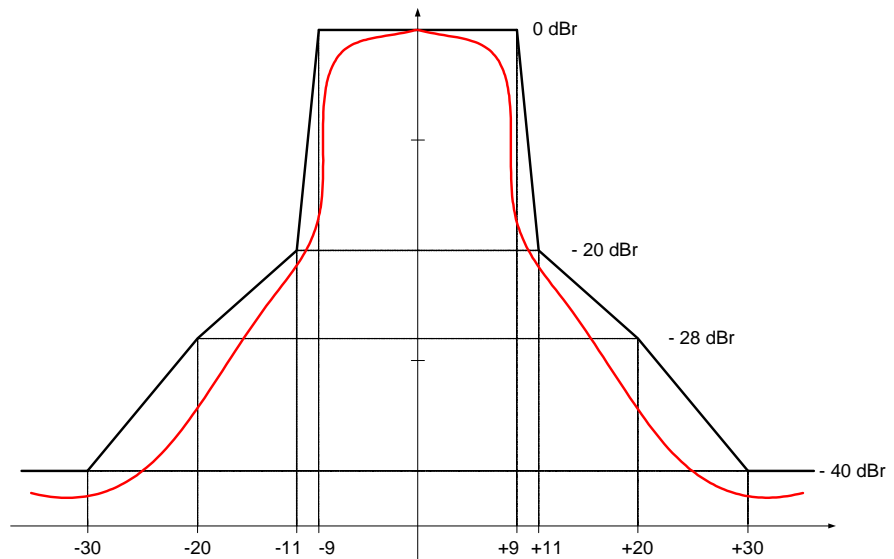
Figure 13 – 802.11a Transmit spectrum mask specification
