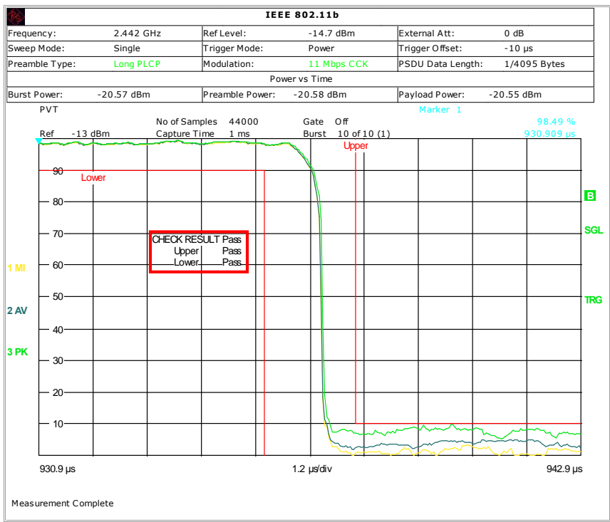
Figure 32 – Transmit power ramp typical measurement result (power-down ramp)
