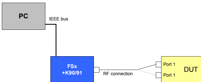
Drawing 10 – Constellation error test setup
