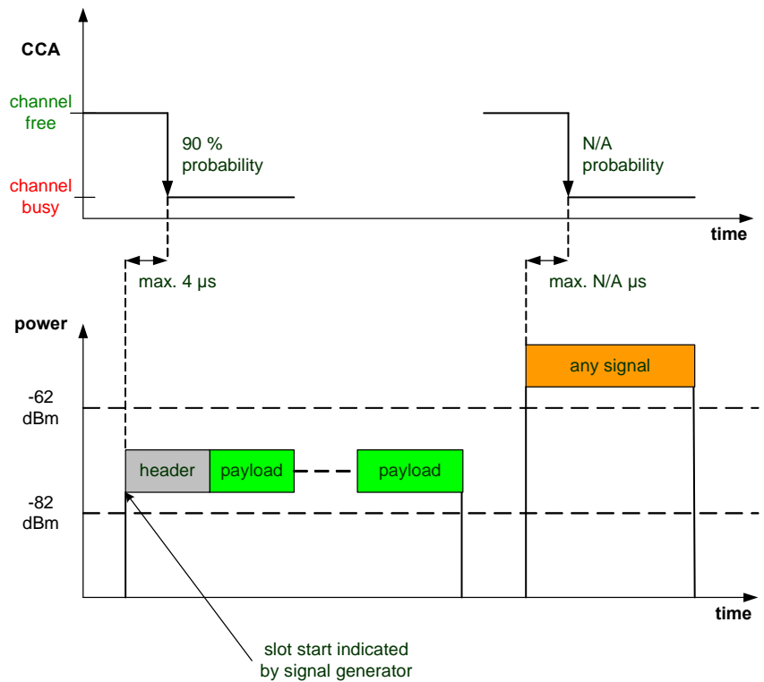
Figure 21 – CCA sensitivity timing overview
