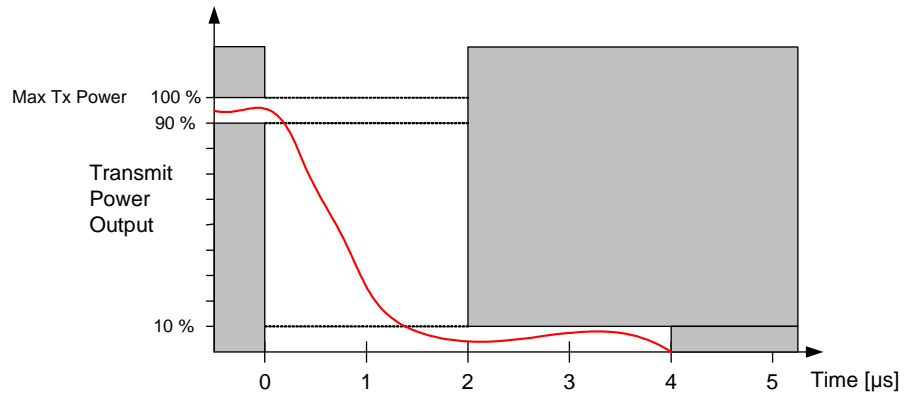
Figure 30 – 802.11b Power-down ramp specification
