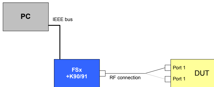
Drawing 7 – Symbol clock tolerance test setup
