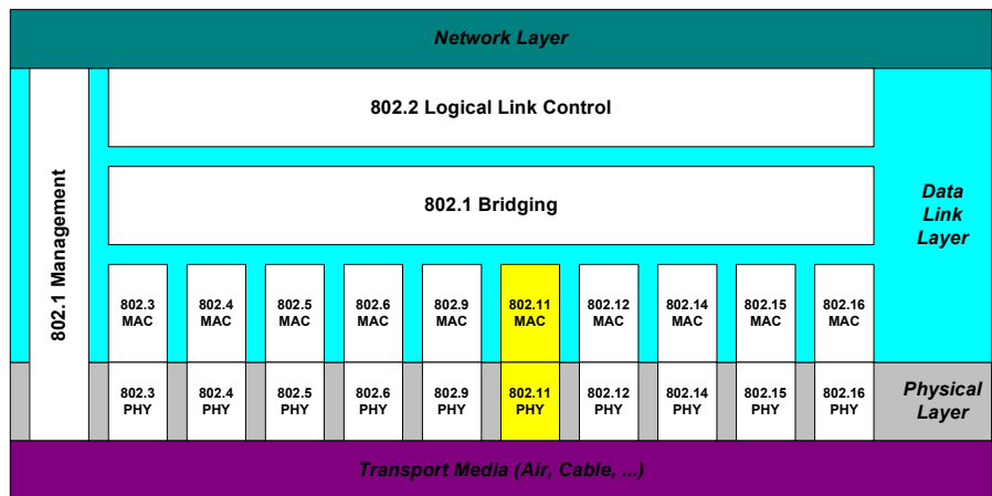
Figure 2 – 802 Standards in the OSI context
