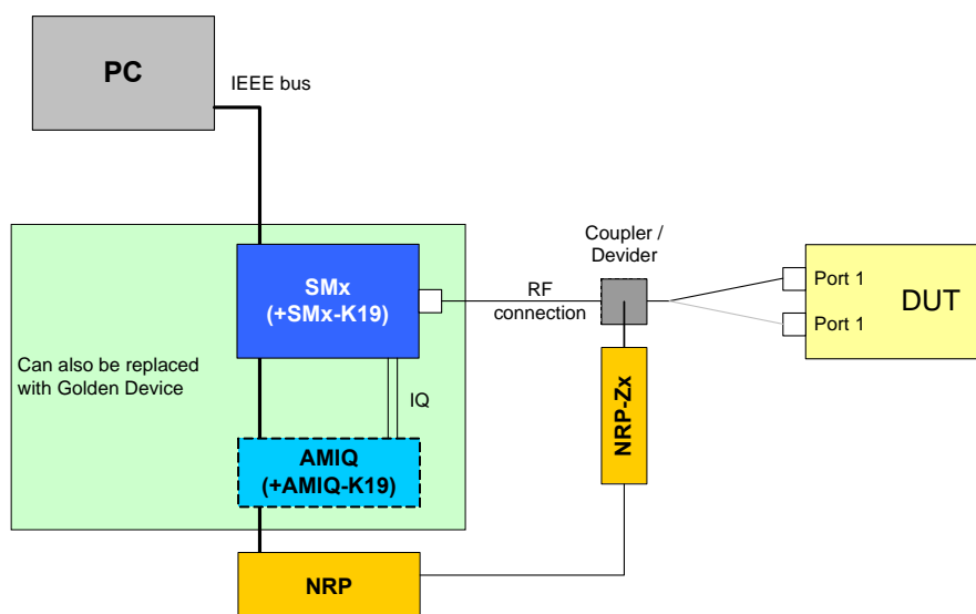
Drawing 26 – Receiver maximum input level test setup
