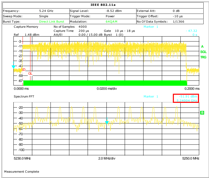
Figure 18 – Transmit center frequency leakage measurement result (using WLAN personality)
