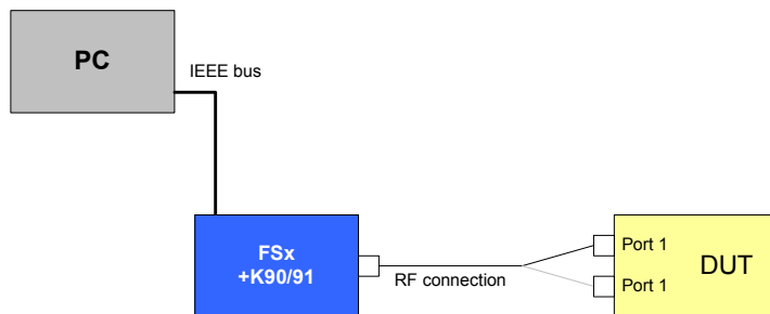
Drawing 11 – Modulation accuracy test setup
