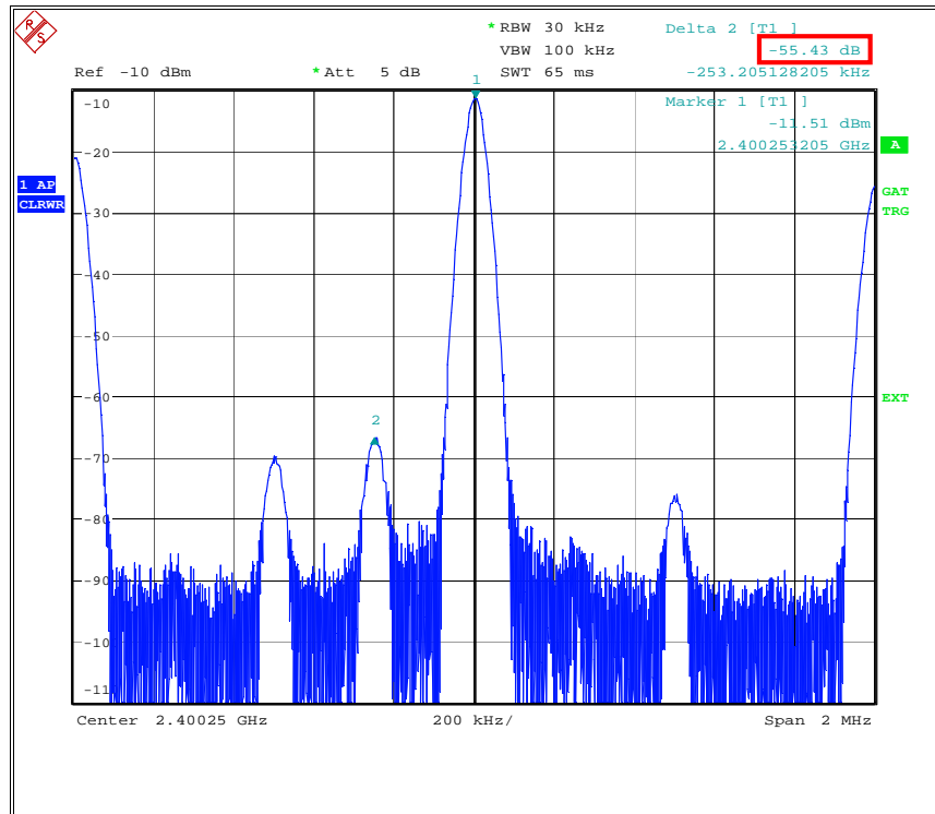
Figure 34 – RF carrier suppression typical measurement result (spectrum analyzer mode)
