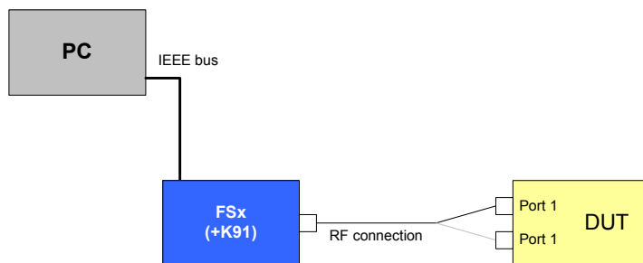
Drawing 19 – Transmit spectrum mask test setup
