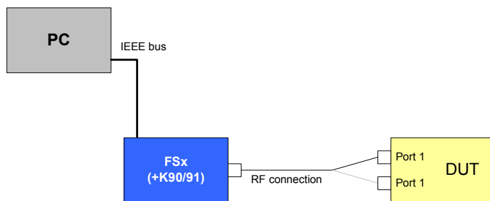
Drawing 1 – Occupied Bandwidth test setup
