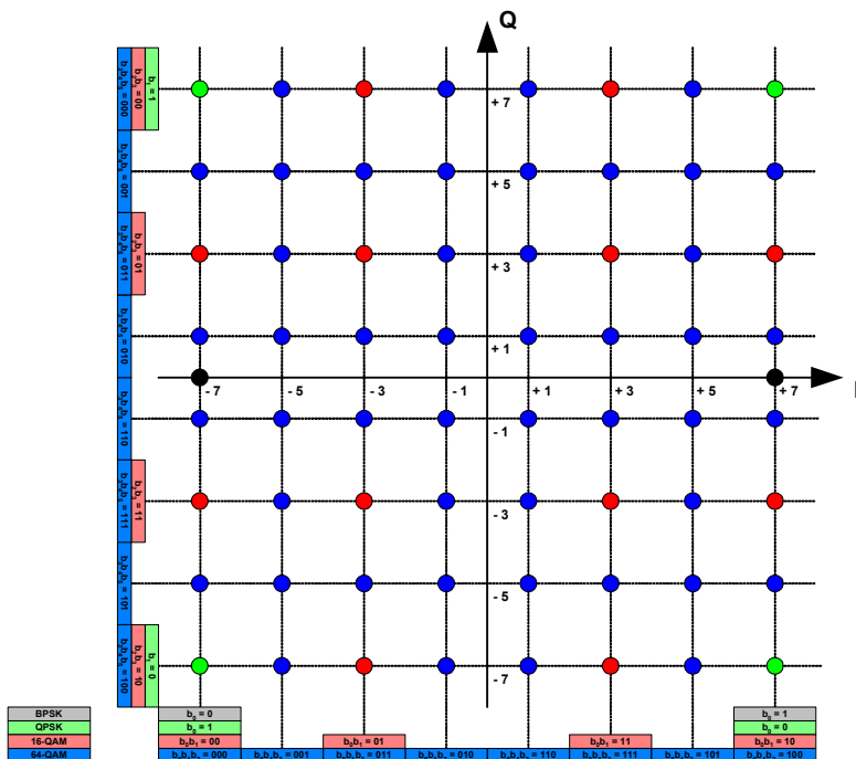
Figure 5 – 802.11a carrier constellations
