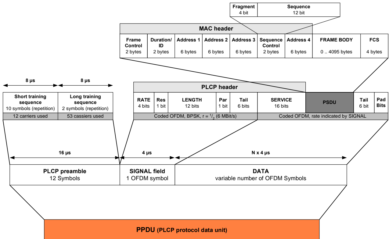
Figure 8 – 802.11a packet format
