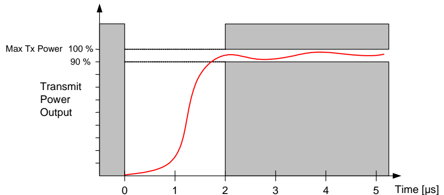
Figure 29 – 802.11b Power-up ramp specification
