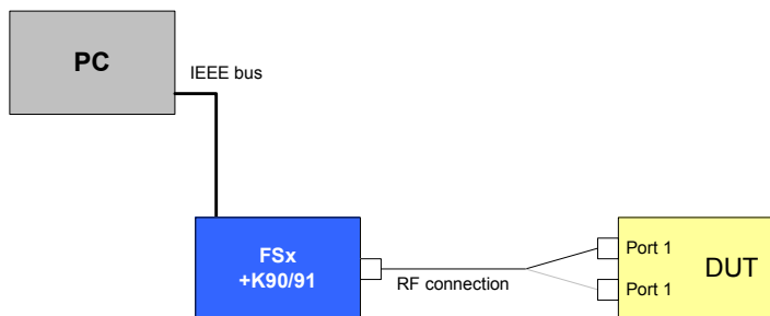
Drawing 9 – Transmit spectrum flatness test setup
