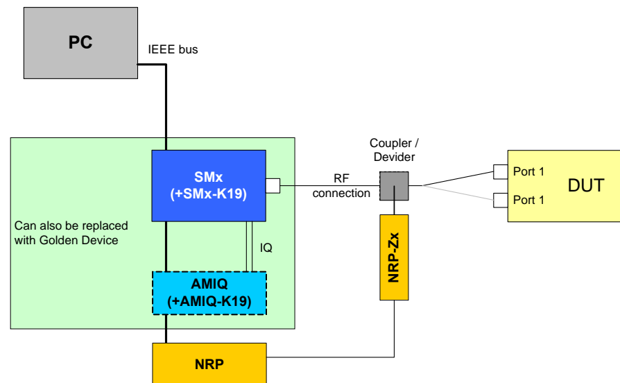
Drawing 12 – Receiver minimum input level test setup
