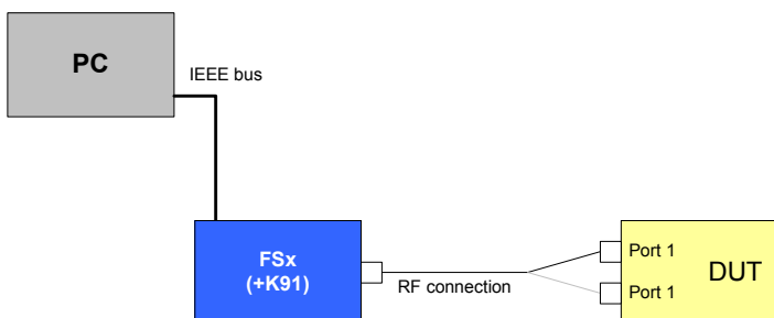
Drawing 18 – Transmit power level control test setup
