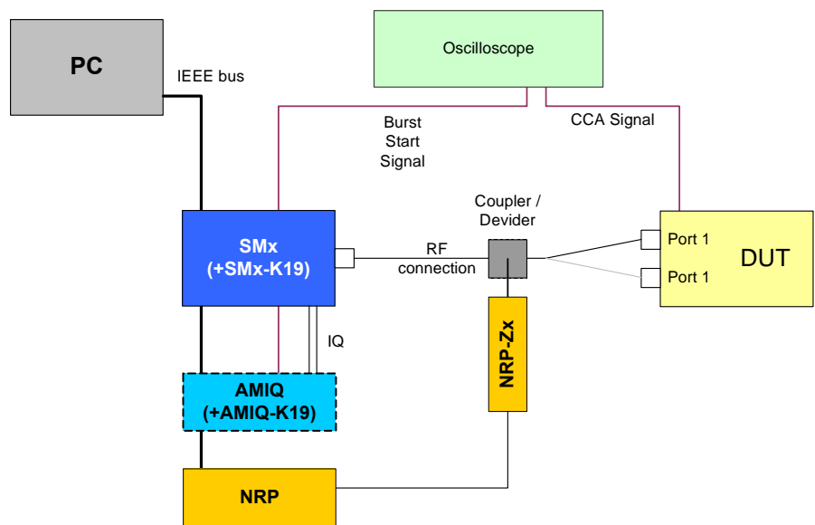
Drawing 16 – CCA sensitivity test setup
