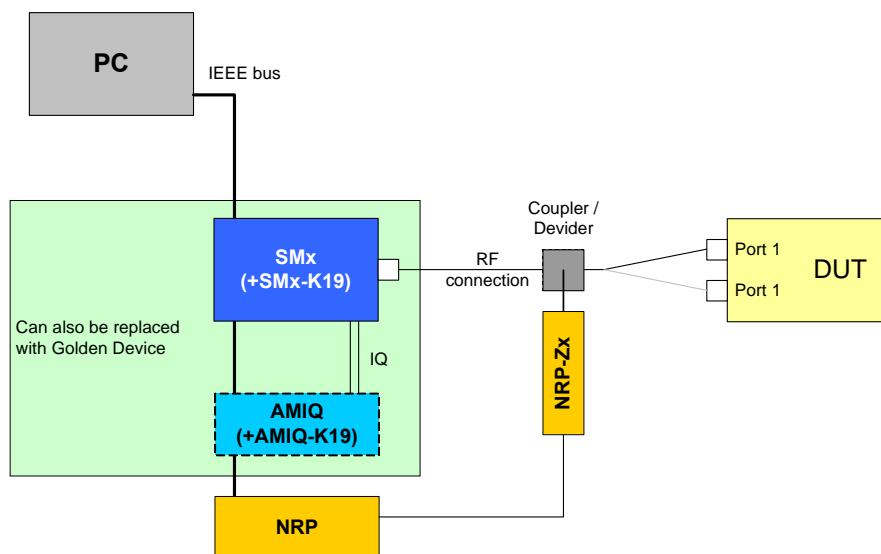
Drawing 25 – Receiver minimum input level sensitivity test setup
