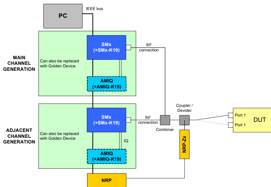
Drawing 13 – Adjacent channel rejection test setup
