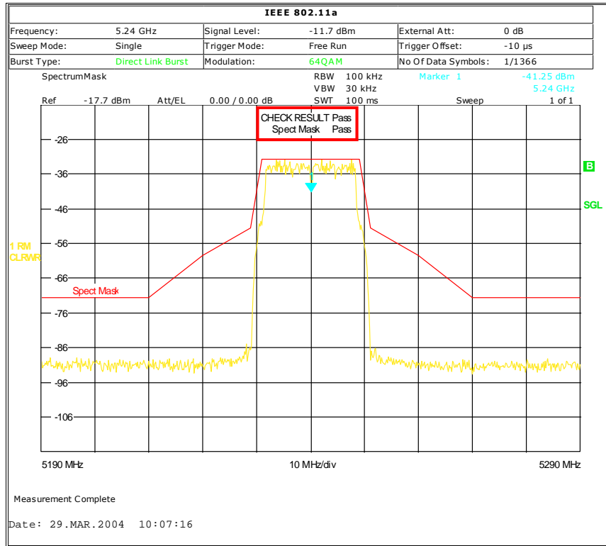
Figure 14 – Transmit spectrum mask measurement result
