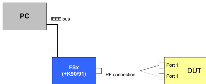
Drawing 3 – Maximum transmit power level test setup
