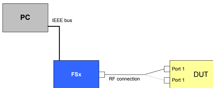
Drawing 2 – Spurious emissions test setup 1)
