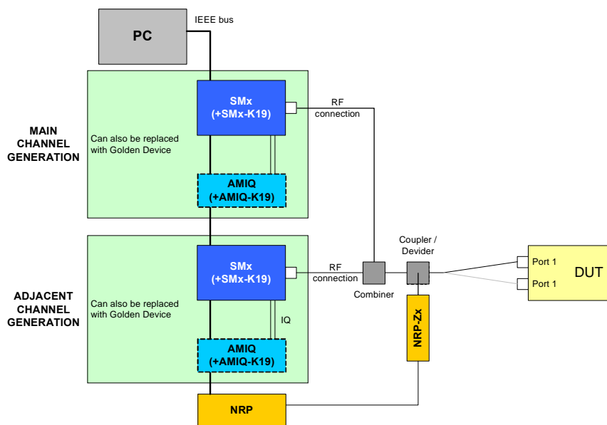
Drawing 27 – Receiver adjacent channel rejection test setup
