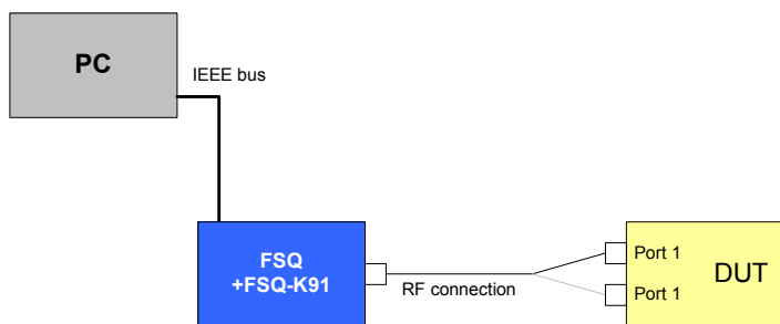
Drawing 21 – Chip clock frequency tolerance test setup
