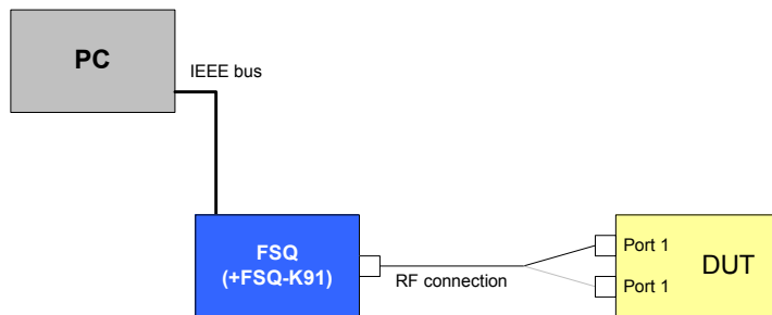
Drawing 22 – Transmit power ramps test setup
