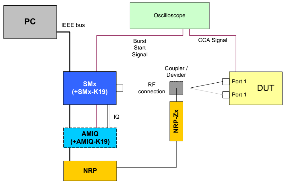
Drawing 28 – CCA test setup
