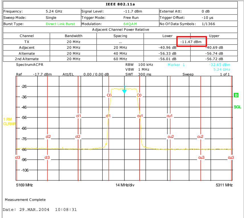
Figure 12 – Maximum transmit power level typical measurement result (using WLAN personality)
