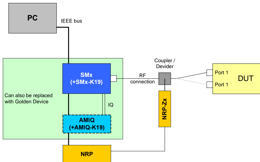
Drawing 15 – Receiver maximum input level test setup
