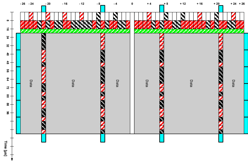
Figure 4 – 802.11a spectrogram representation (carriers vs time)
