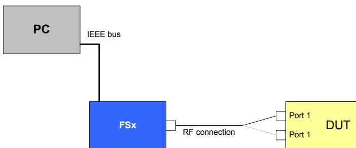
Drawing 5 – Transmit spurious test setup 1)
