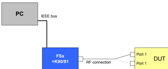
Drawing 6 – Center frequency tolerance test setup
