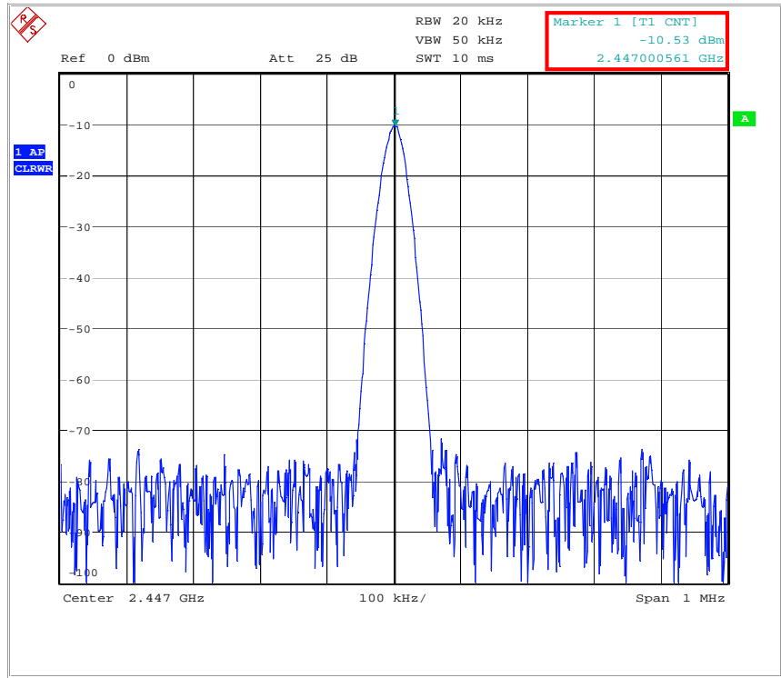
Figure 27 – Transmit center frequency error typical measurement result – counter measurement
