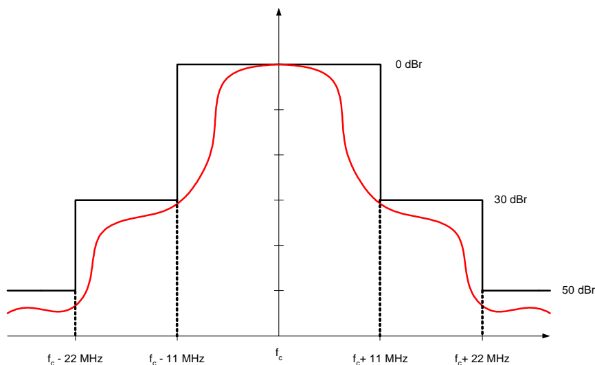
Figure 24 - 802.11b Transmit Spectrum Mask Specification
