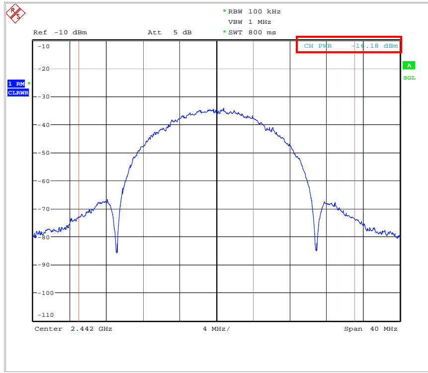
Figure 22 – Transmit power levels typical measurement result (using spectrum analyzer function)
