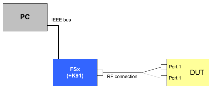
Drawing 17 – Transmit power levels test setup
