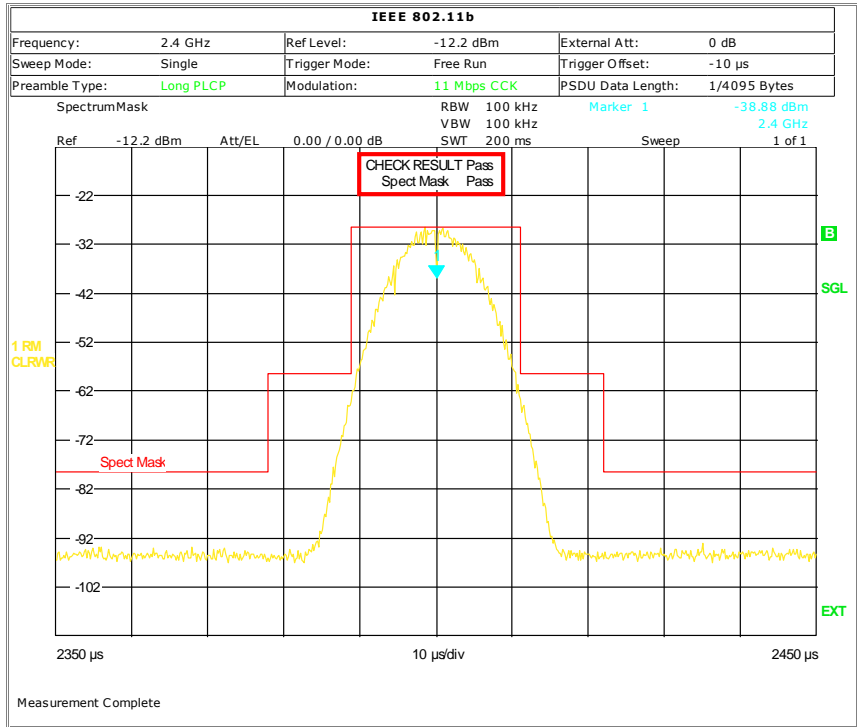
Figure 25 – Transmit spectrum mask typical measurement result
